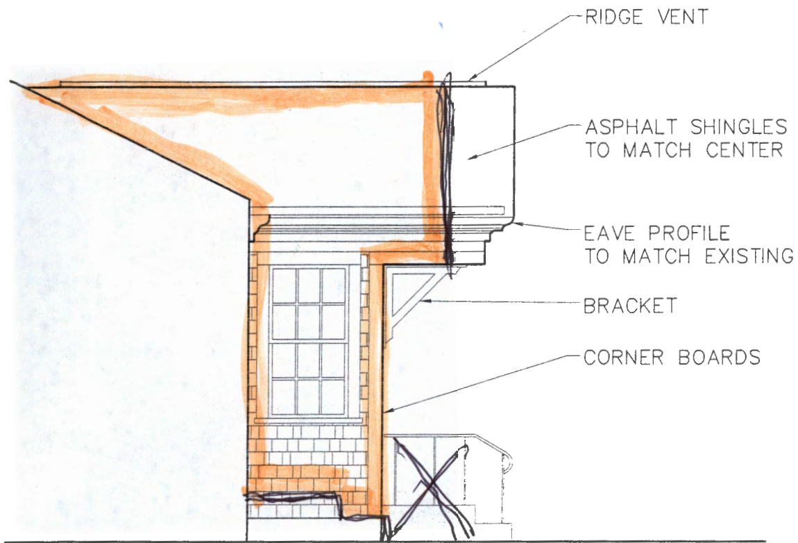
8 SIDE ELEVATION (BOTH SIDE TYPICAL)
